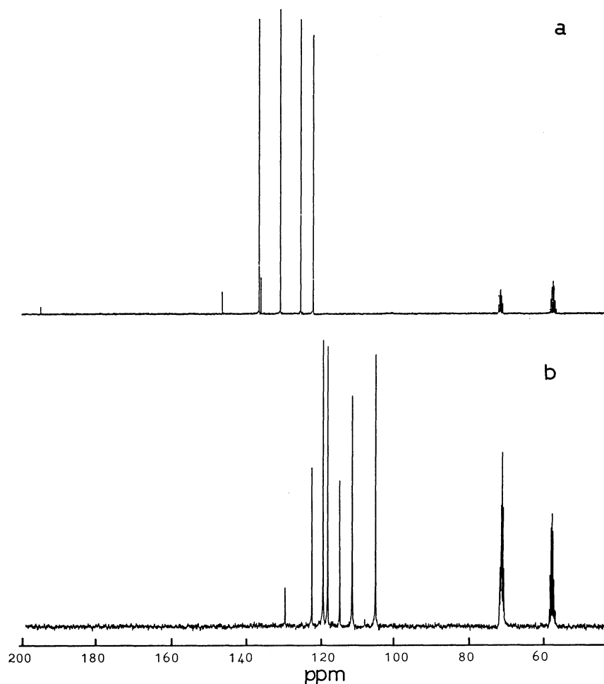
Fig. 2. ^{13}\text{C} NMR spectra (75 MHz) of fluorenone in \text{DME-d}_{10} (a) and of the diamagnetic green species formed by sodium reduction in \text{DME-d}_{10} (b).
